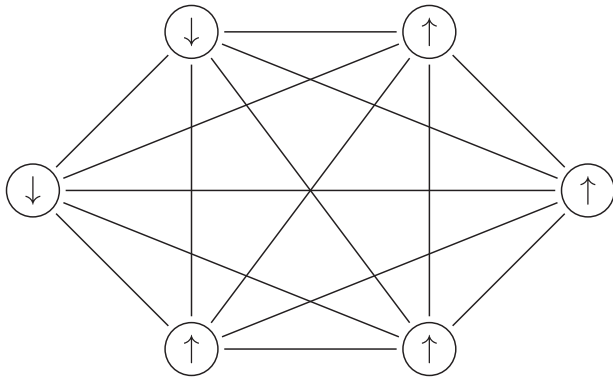
Figure 5. A graphical representation of the Curie-Weiss network. The nodes (circles) refer to the upward “↑” and downward “↓” orientation of particles and each particle interacts with each other particle (solid lines).
