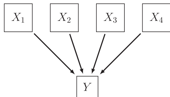
Figure 11. A graphical representation of the common effect model. The observables X are the collective cause of the effect Y .
