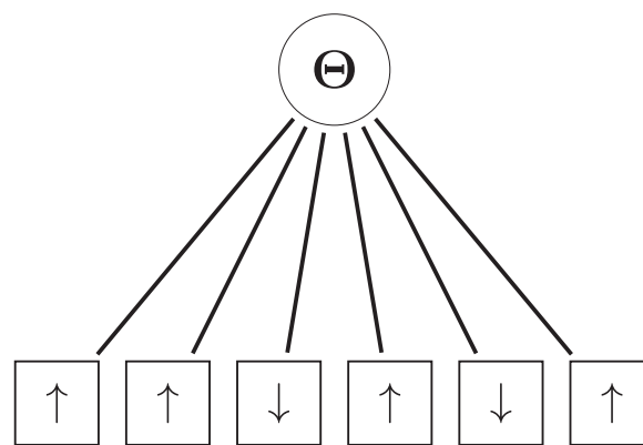
Figure 6. A graphical representation of the Rasch model. The observables (squares) refer to the upward “↑” and downward “↓” orientation of particles and each particle interacts with another particle only through the latent variable \Theta .
